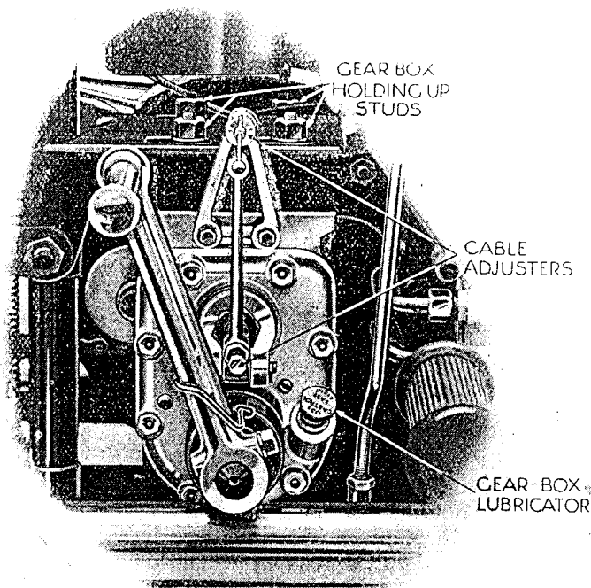
FIG. 57. THE HEAVYWEIGHT 3-SPEED GEAR-BOX (MODELS TB8, T9)
