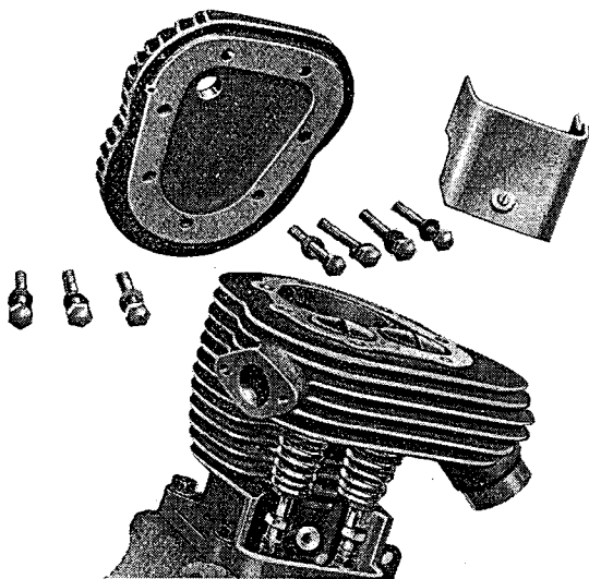
FIG. 16A. THE CAR TYPE DETACHABLE CYLINDER HEAD ON THE 4.98 H.P. S.V. MODEL
