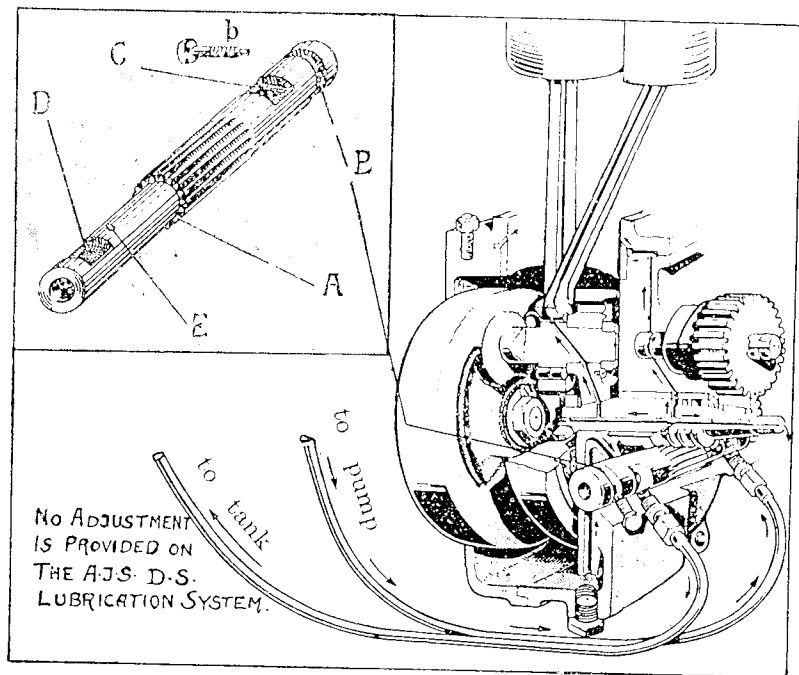
FIG. 41A. DIAGRAM SHOWING THE OIL CIRCULATION IN THE DRY SUMP LUBRICATION SYSTEM USED ON THE 1933 BIG TWINS
