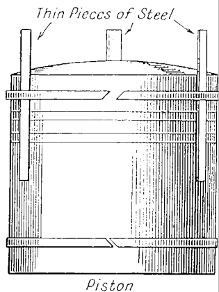
FIG. 51. HOW TO REMOVE PISTON RINGS
