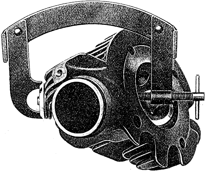
FIG. 47. THE A.J.S. OVERHEAD VALVE EXTRACTOR
