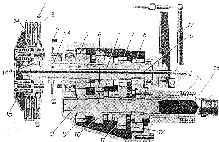
FIG. 42. SECTIONAL ARRANGEMENT OF STURMEY-ARCHER HEAVYWEIGHT 4-SPEED GEAR-BOX AND 3-PLATE CLUTCH
