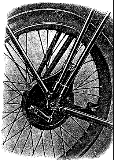
FIG. 5. HOW THE CABLE TO THE FRONT BRAKE ANCHOR PLATE LEVER IS LED FROM THE HANDLEBARS
