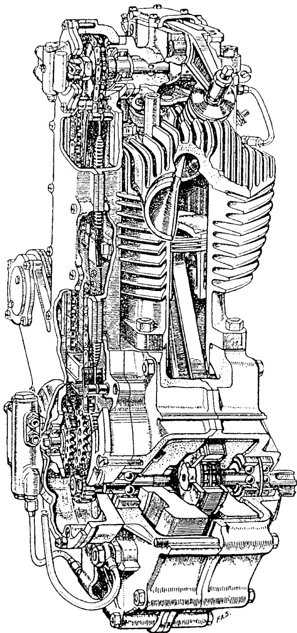
FIG. 46. PARTLY SECTIONED VIEW OF THE 1933 O.H.C. ENGINE
