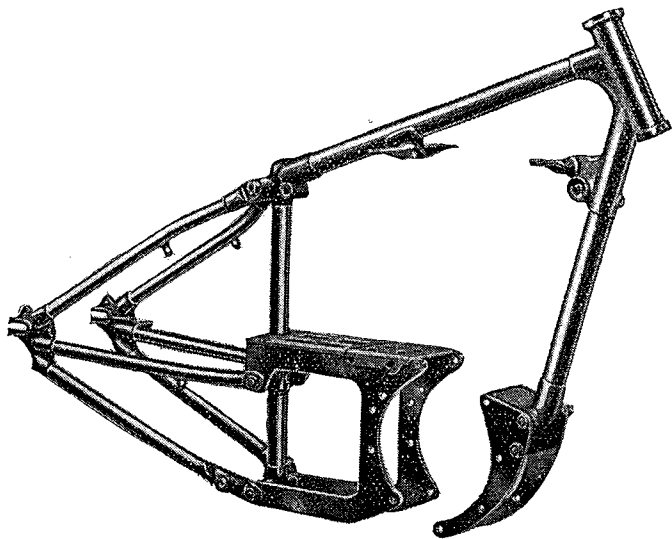
FIG. 12. THE STURDY SEMI-CRADLE FRAME
