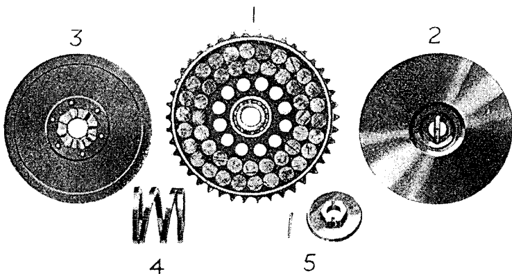
FIG. 59. LIGHTWEIGHT CLUTCH PARTS (1927-29)
