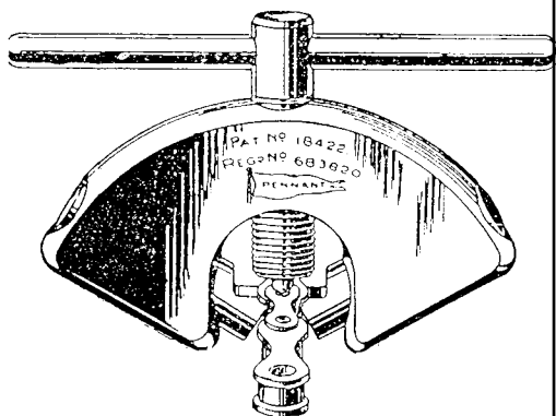
FIGS. 61, 62. CHAIN REPAIR PARTS AND RIVET EXTRACTOR
