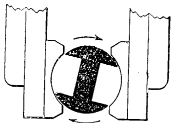
FIG. 33. POSITION OF MAGNETO ARMATURE WHEN CONTACTS SHOULD OPEN
