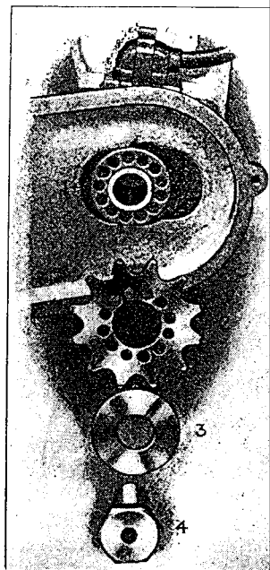
FIG. 53. THE VERNIER TIMING ADJUSTMENT
