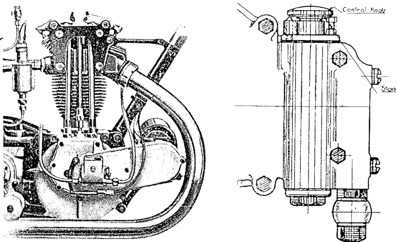
FIG. 22. SHOWING PUMP UNIT AND OIL SUPPLY CONTROL
