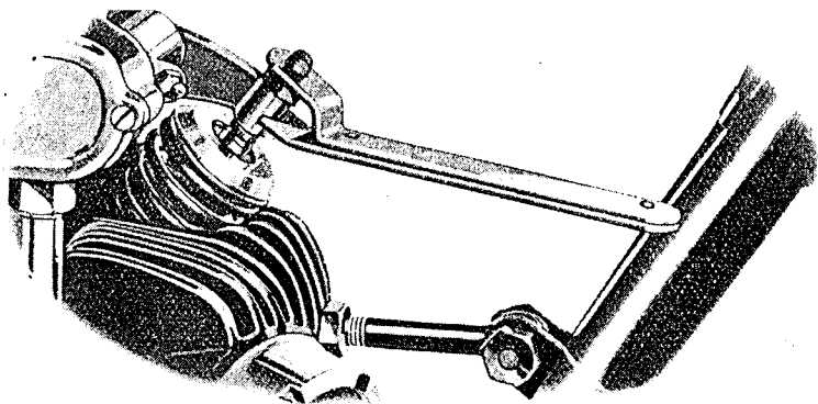
FIG. 45A. THE A.J.S. PUSH-ROD EXTRACTOR
