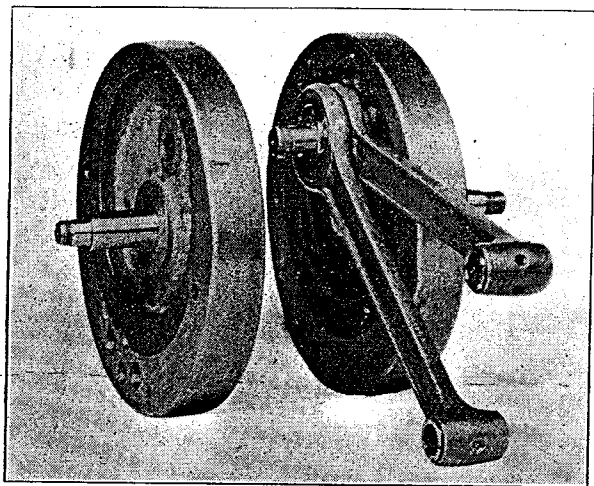
FIG. 18. CONNECTING-ROD MOUNTING ON TWIN CYLINDER ENGINES
