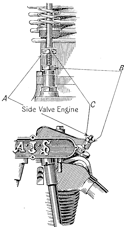
FIG. 45. VALVE CLEARANCE ADJUSTMENT
