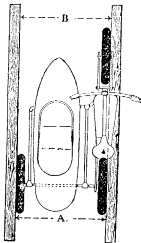
FIG. 66. SIDECAR ALINEMENT The distances A and B must be equal
