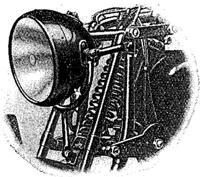
FIG. 14A. SHOWING A.J.S. FORK SUSPENSION AND HEADLAMP MOUNTING
