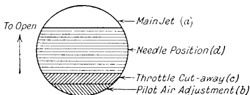
FIG. 56. RANGE AND SEQUENCE OF AMAL ADJUSTMENTS
