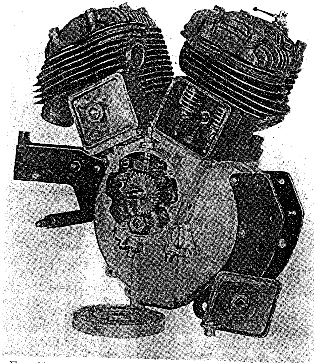
FIG. 19. CLOSE-UP VIEW OF THE 9-90 H.P. 33/2 ENGINE
