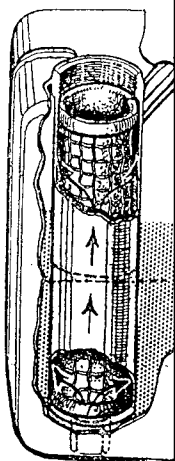
FIG. 18A. FABRIC FILTER
