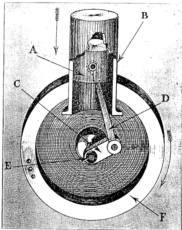
FIG. 28. DIAGRAM ILLUSTRATING HOW A PISTON (A), SLIDING IN A CYLINDER (B), ROTATES THE FLYWHEEL (F)
