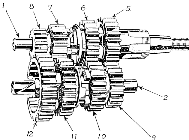
FIG. 42A. THE STURMEY-ARCHER 4-SPEED TRAIN OF PINIONS
