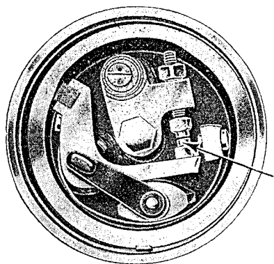
FIG. 52. THE CONTACT-BREAKER
