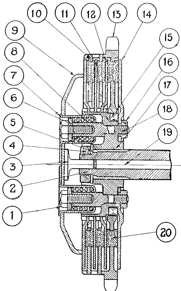
FIG. 58. SECTIONAL VIEW OF A.J.S. HEAVYWEIGHT MULTI-PLATE CLUTCH (3- AND 4-SPEED HEAVYWEIGHT MODELS)
