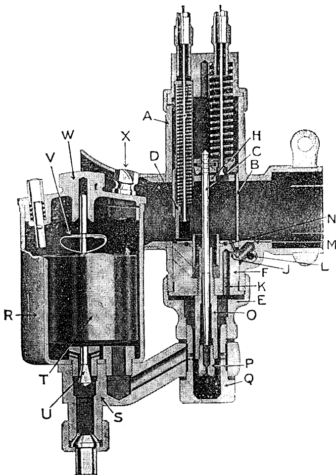
FIG. 36. SECTIONAL VIEW OF AMAL SEMI-AUTOMATIC TWO-LEVER CARBURETTOR
