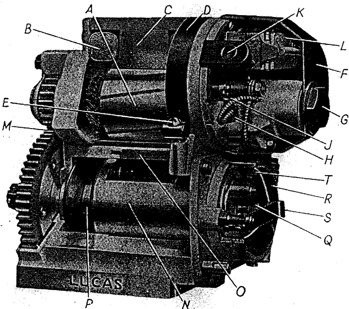
FIGS. 67, 68. SHOWING (ABOVE) CONTACT-BREAKER SIDE OF LUCAS "MAGLITA" AND (BELOW) SECTIONAL VIEW OF LUCAS "MAGDYNQ"
