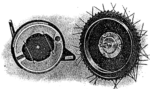
FIG. 13. SHOWING REAR BRAKE DRUM AND ANCHOR PLATE WITH SHOES
